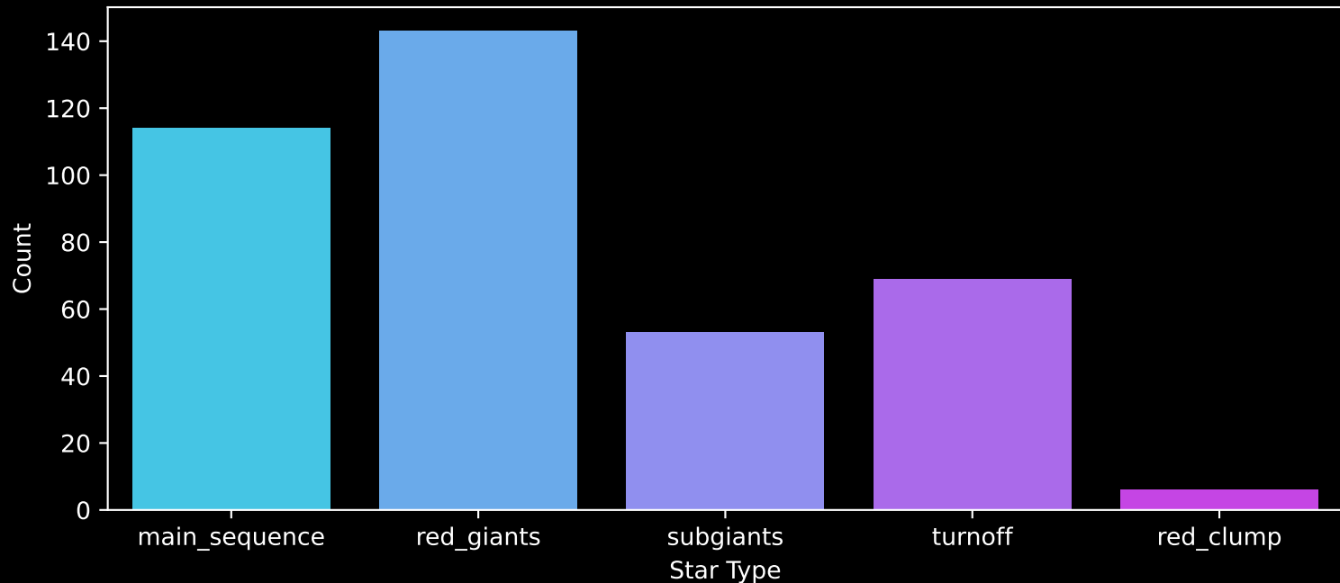
APOGEE DR17 Field: [PAL5-1] Count plot of Star Type
