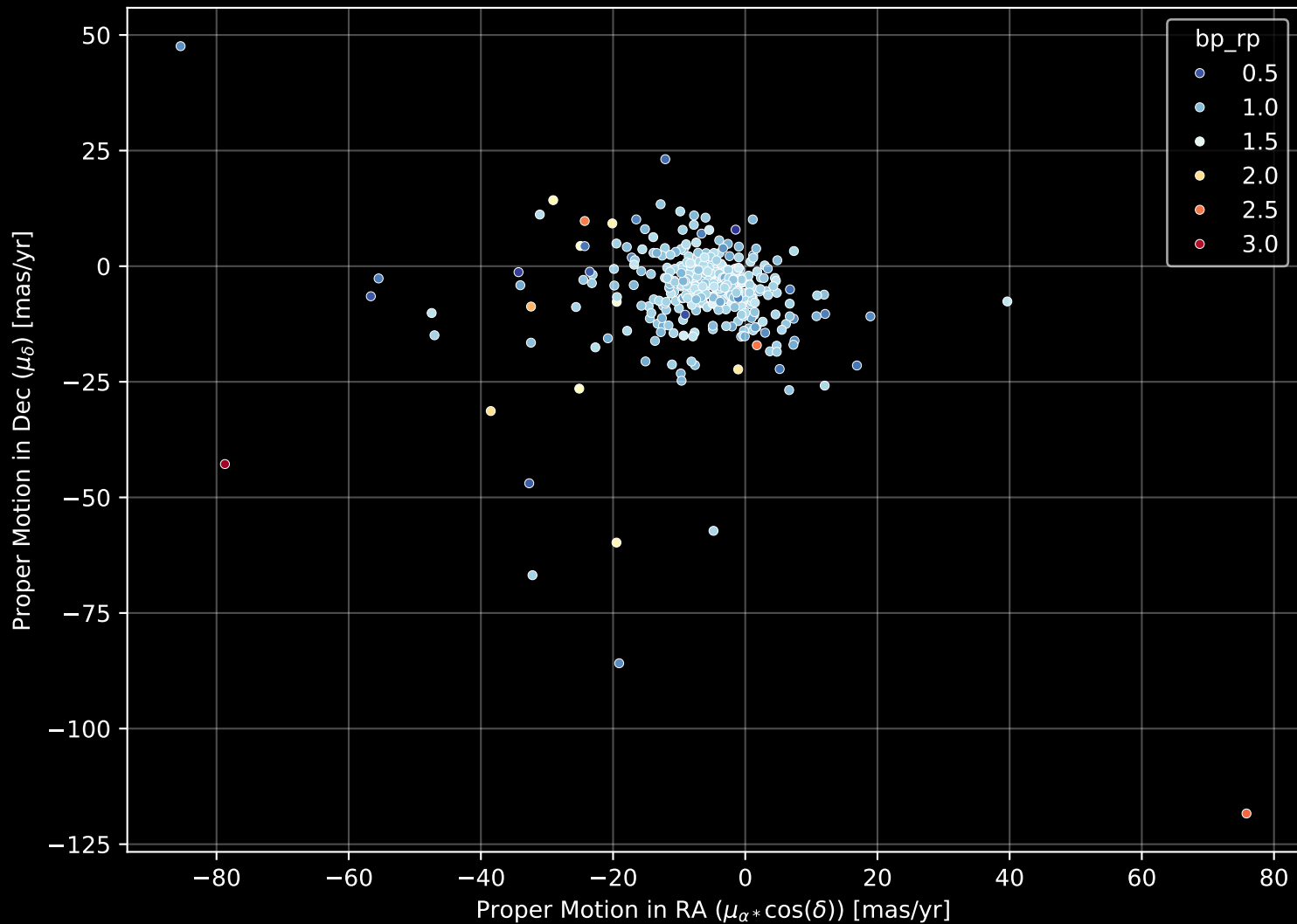
APOGEE DR17 Field: [PAL5-1] Proper Motion Diagram (n= 385)
