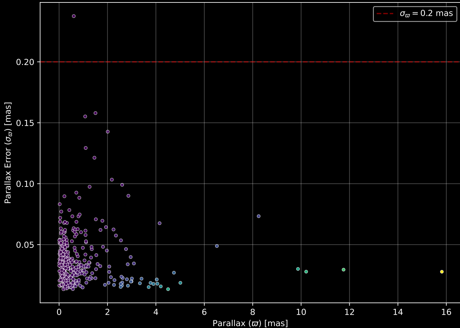
APOGEE DR17 Field: [PAL5-1] Parallax Quality (n= 385)
