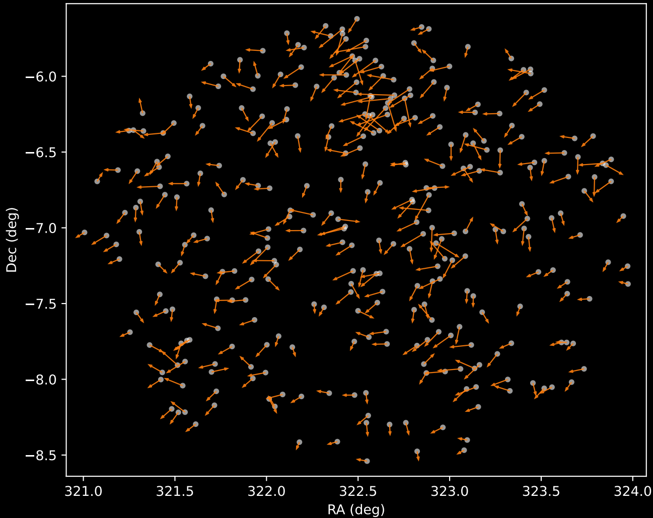
APOGEE DR17 Cluster 2 Proper Motion Vectors (n=323)
