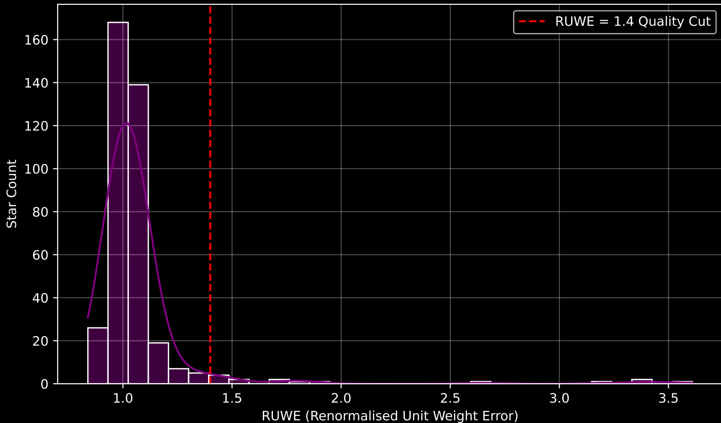
GAPOGEE DR17 Field [PAL5-1] RUWE Distribution (n= 379)
