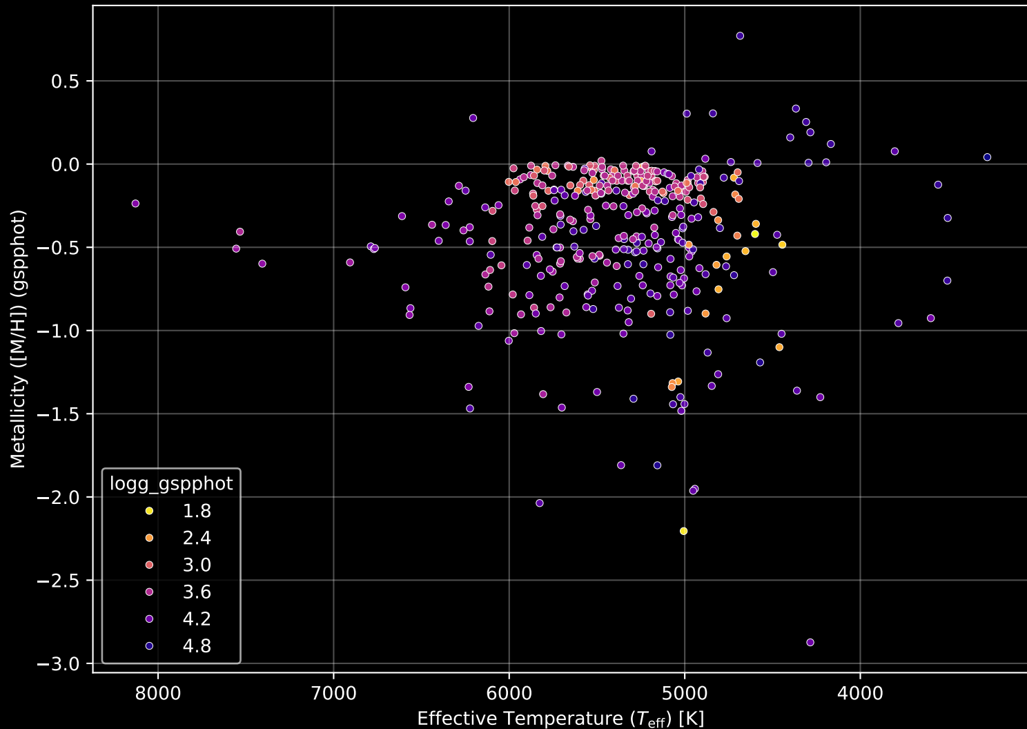
APOGEE DR17 Field: [PAL5-1] Stellar Population Parameters (n= 385)
