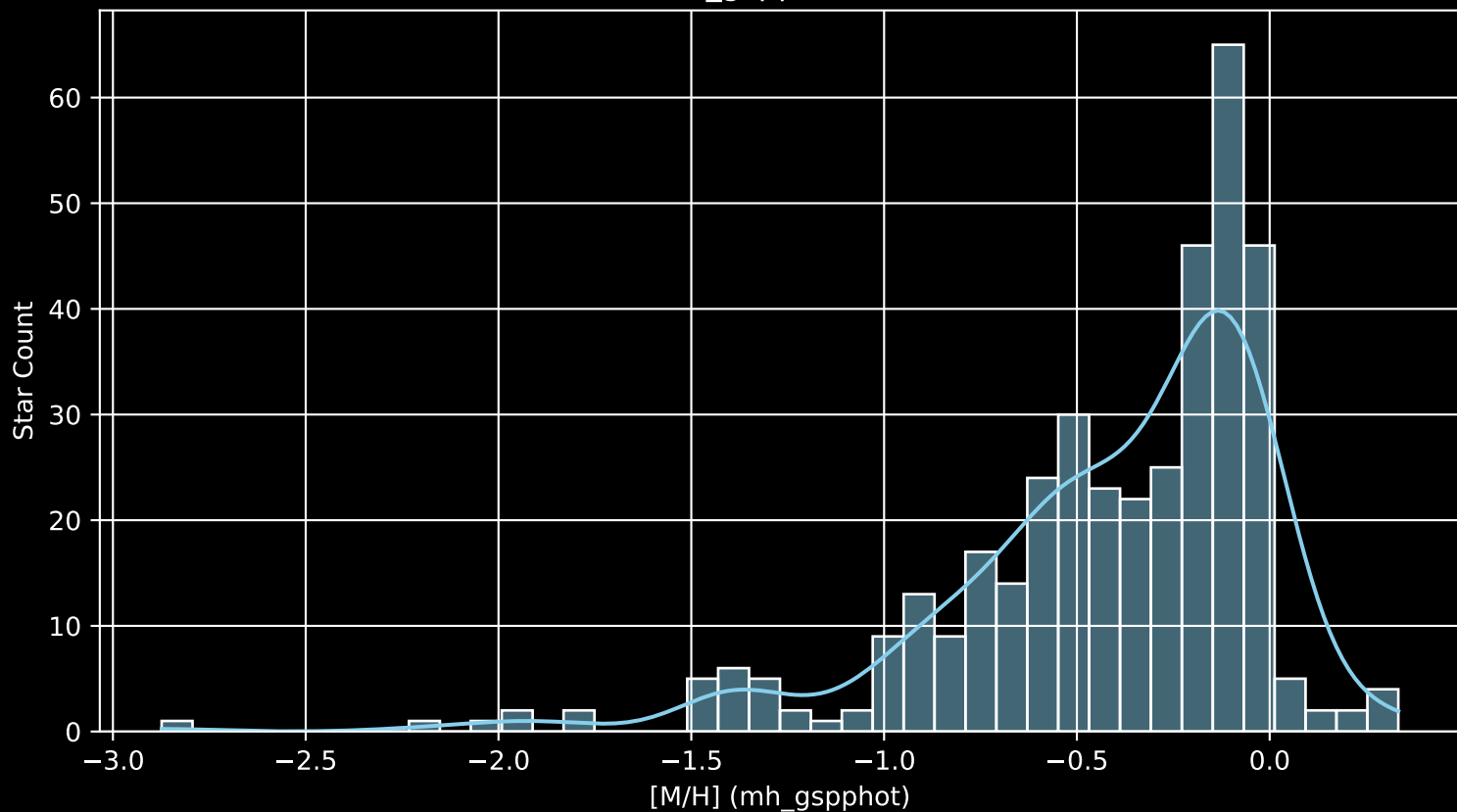
APOGEE DR17 Field: [PAL5-1 [M/H] (mh_gspphot) (n= 384)
